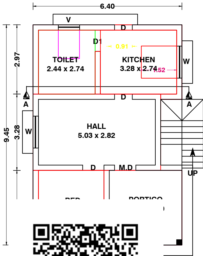
FLOOR PLAN
