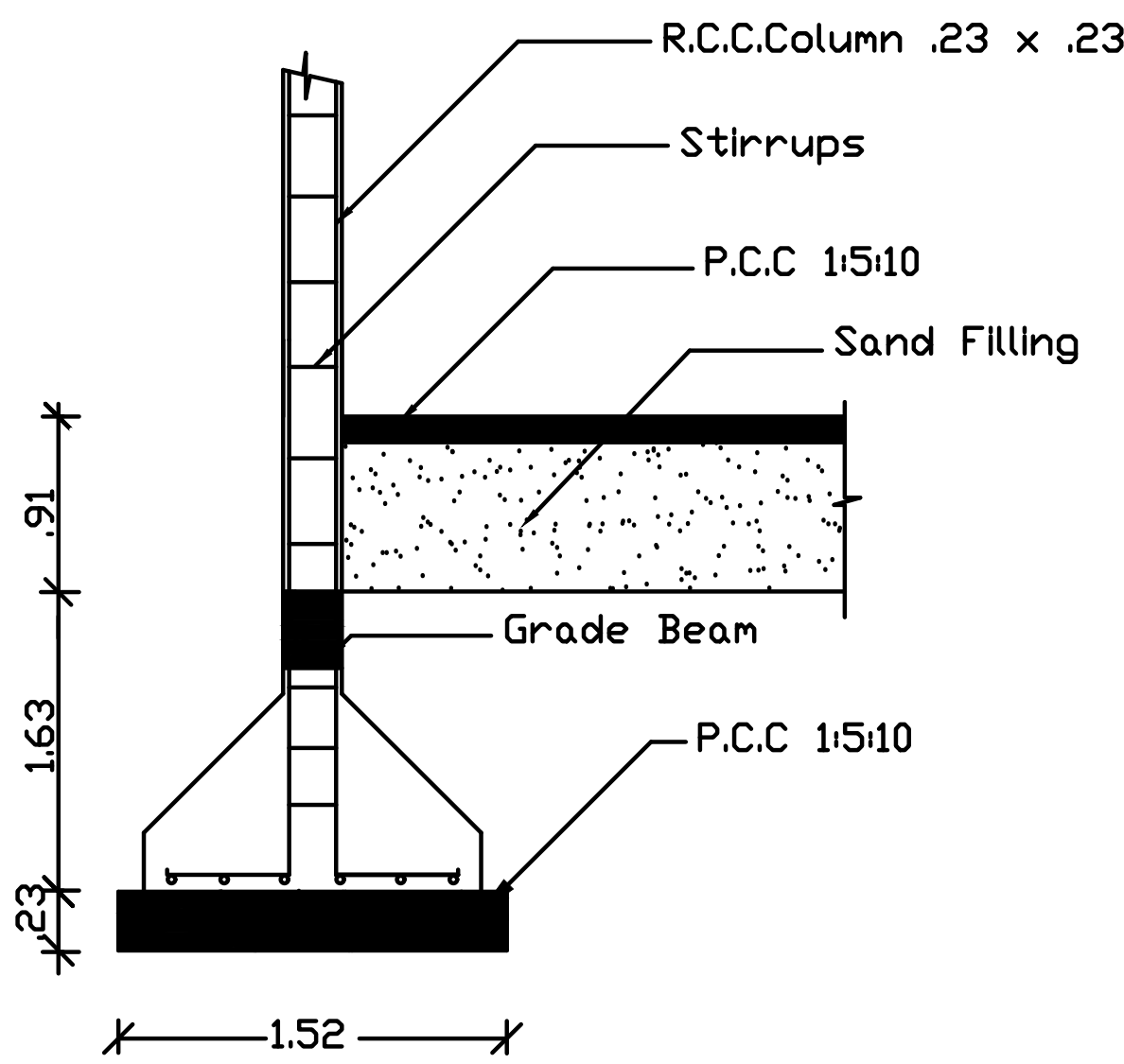
COLUMN DETAIL
