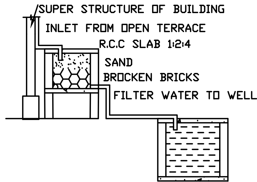
RAINWATER HARVESTING
