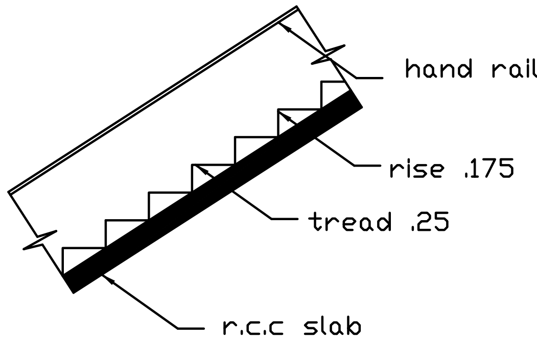
STAIR
