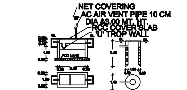
PLAN AND CROSS SECTION OF ST&SP
