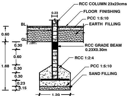
FOUNDATION DETAILS
