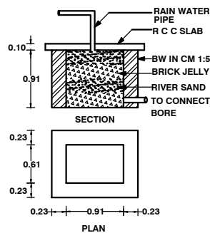
RAIN WATER COLLECTION TANK
