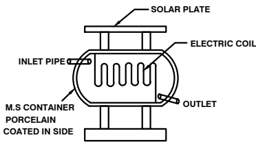
SOLAR SYSTEM
