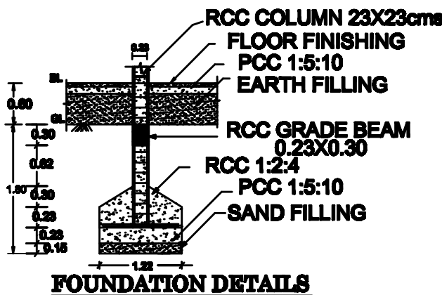
FOUNDATION DETAILS
