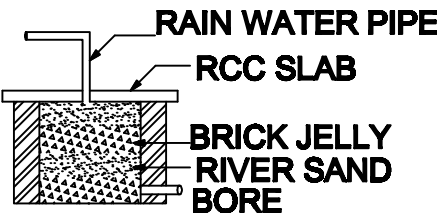
SECTION
