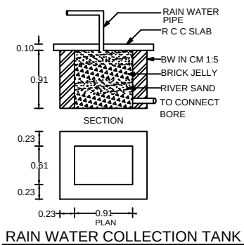
RAIN WATER COLLECTION TANK
