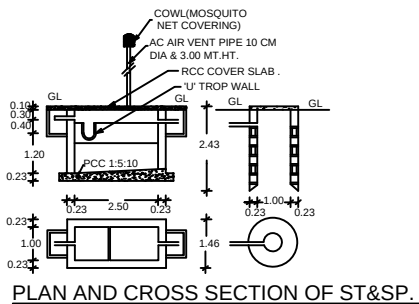
PLAN AND CROSS SECTION OF ST&SP.
