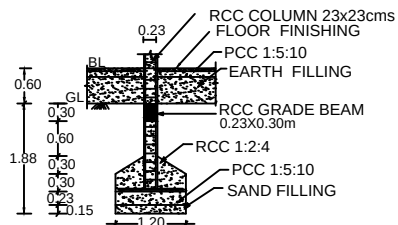
FOUNDATION DETAILS
