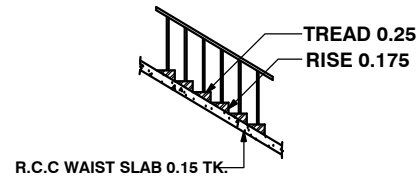
STAIR CASE DETAILS
