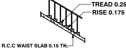
STAIR CASE DETAILS
