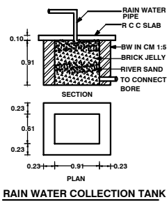
RAIN WATER COLLECTION TANK
