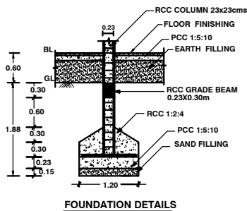
FOUNDATION DETAILS
