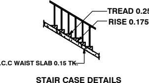
STAIR CASE DETAILS
