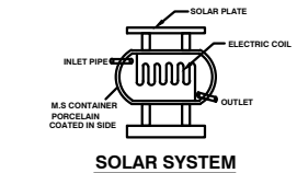
SOLAR SYSTEM
