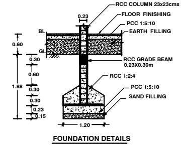
FOUNDATION DETAILS
