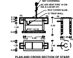
PLAN AND CROSS SECTION OF ST&SP.
