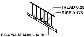
STAIR CASE DETAILS
