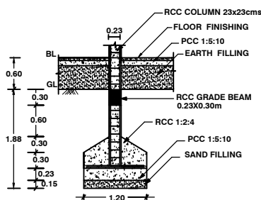
FOUNDATION DETAILS
