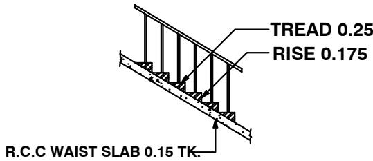
STAIR CASE DETAILS
