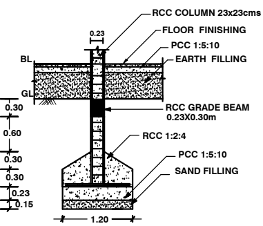
FOUNDATION DETAILS
