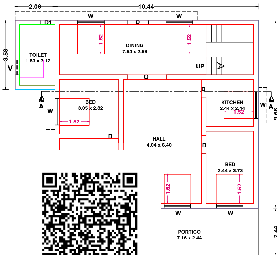
R PLAN
