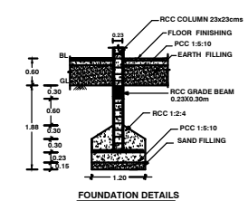
FOUNDATION DETAILS
