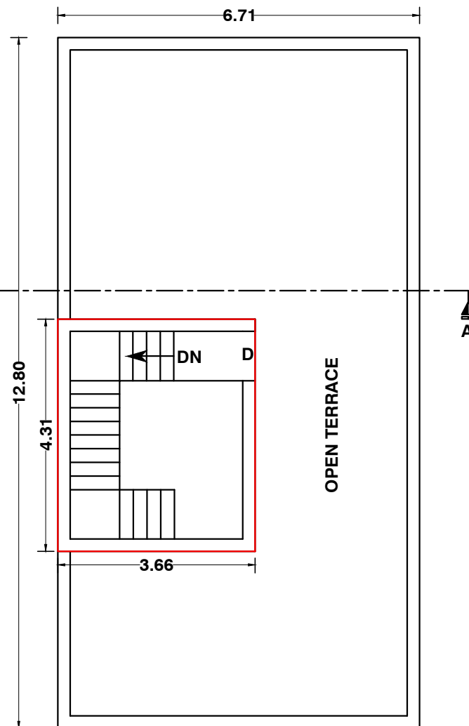
HEAD ROOM PLAN
