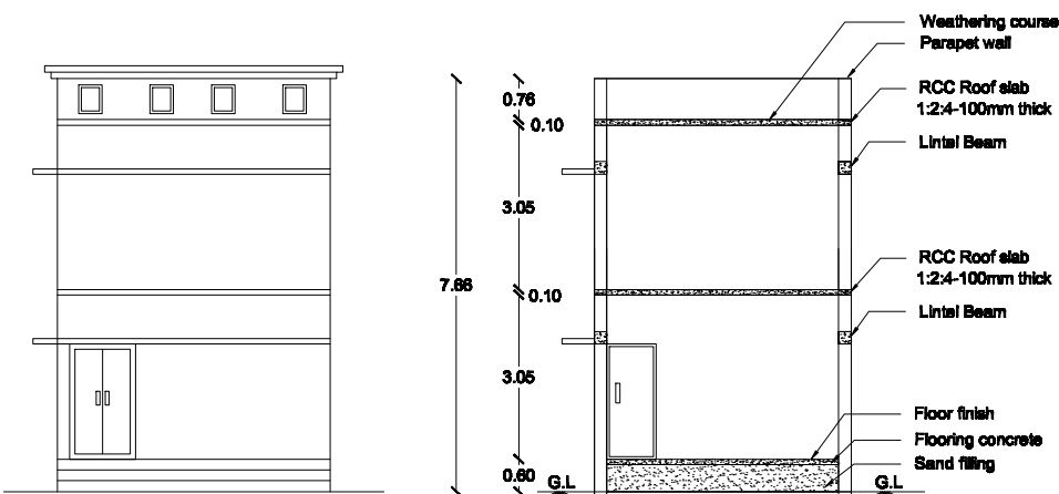
FRONT ELEVATION
