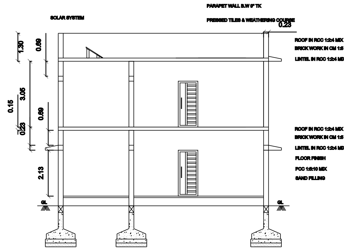
CROSS SECTION AB
