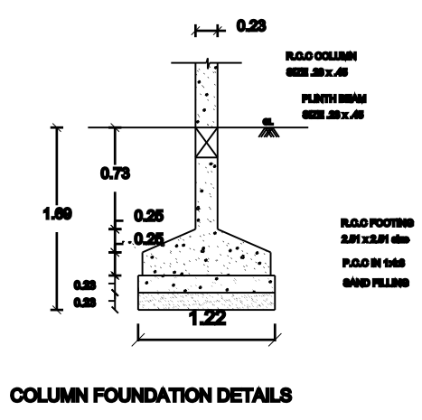
COLUMN FOUNDATION DETAILS
