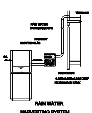
MAIN WATER HARVESTING SYSTEM
