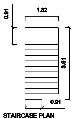
STAIRCASE PLAN
