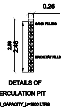
DETAILS OF PERCOLATION PIT
