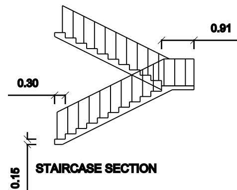
STAIRCASE SECTION
