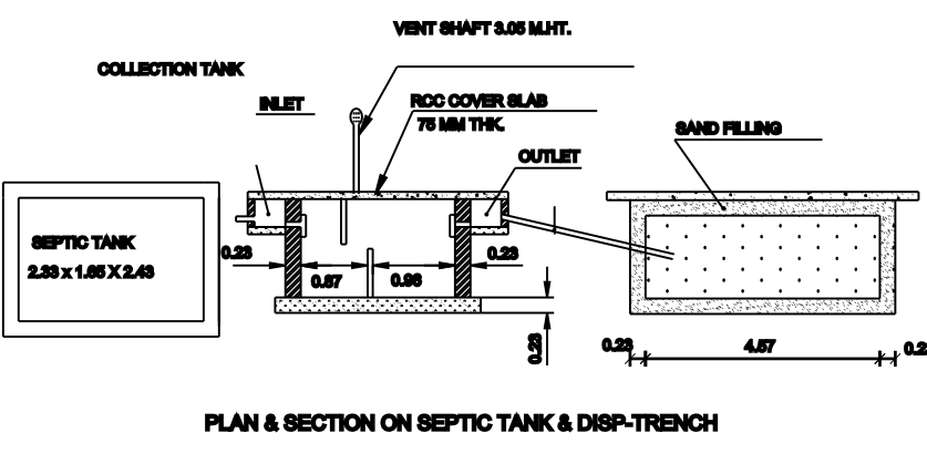
PLAN & SECTION ON SEPTIC TANK & DRAIN TRENCH
