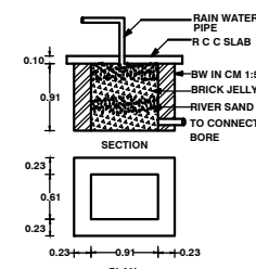
RAIN WATER COLLECTION TANK
