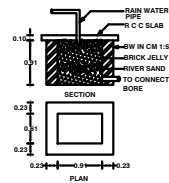
RAIN WATER COLLECTION TANK
