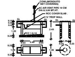
PLAN AND CROSS SECTION OF ST&P.
