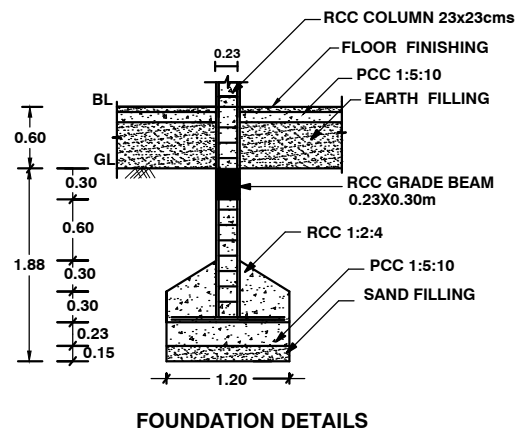
FOUNDATION DETAILS
