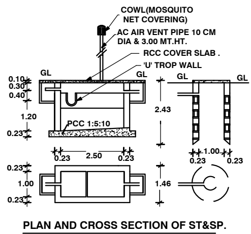
PLAN AND CROSS SECTION OF ST&SP.
