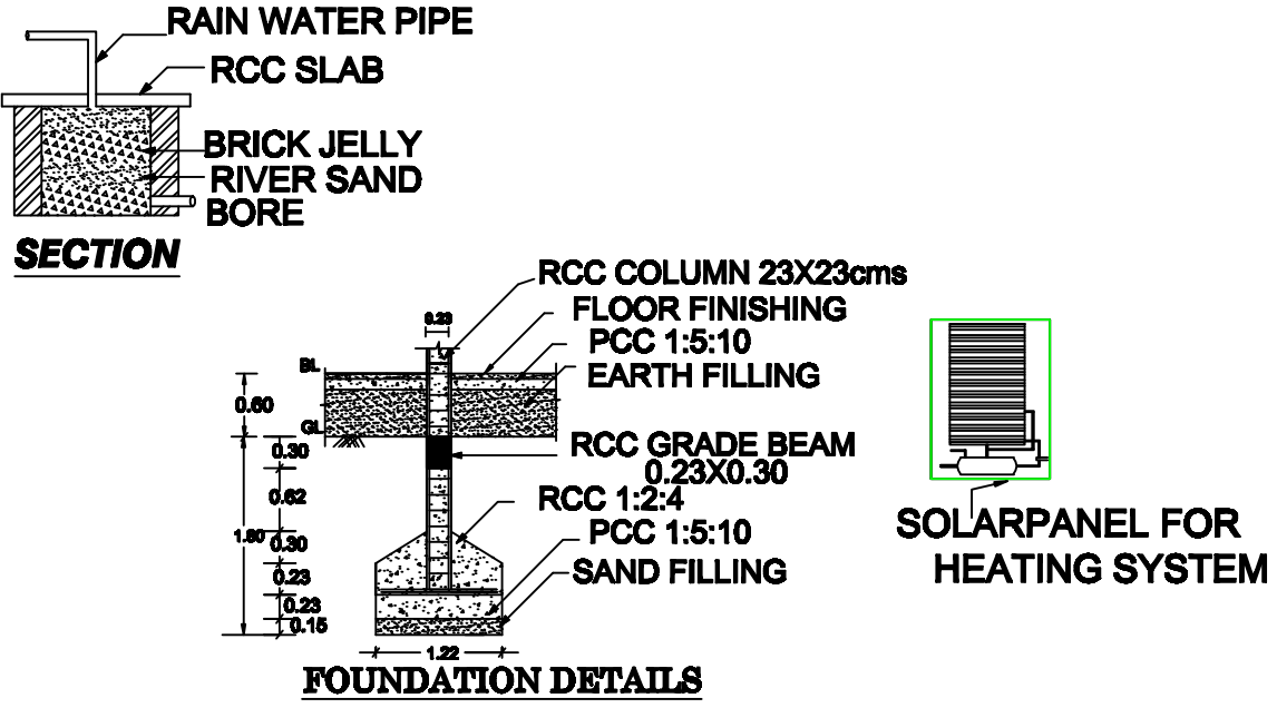
FOUNDATION DETAILS
