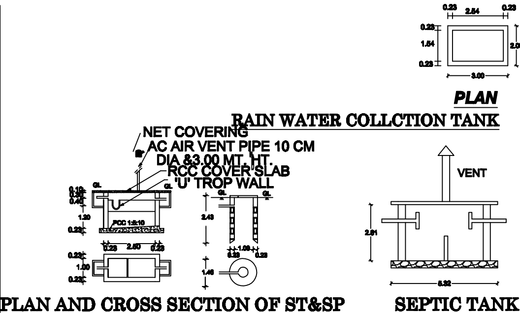
PLAN AND CROSS SECTION OF ST&SP
