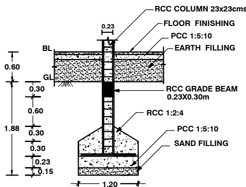
FOUNDATION DETAILS
