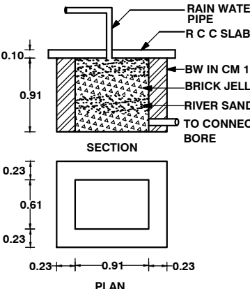
RAIN WATER COLLECTION TANK
