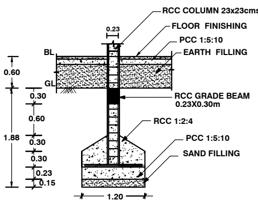
FOUNDATION DETAILS
