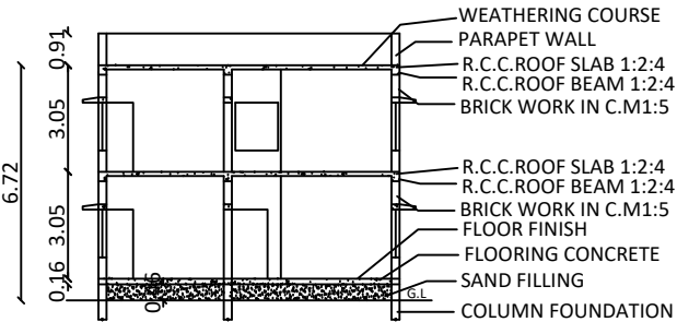
SECTION- SS
