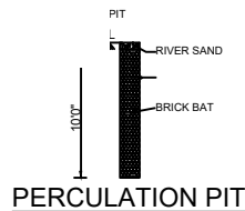
PERCOLATION PIT
