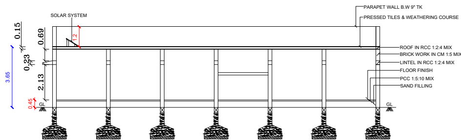
CROSS SECTION AB
