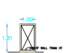
WIKET GATE ELEVATION
