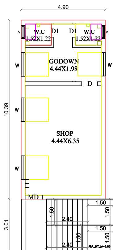
PRO.SECOND FLOOR PLAN
