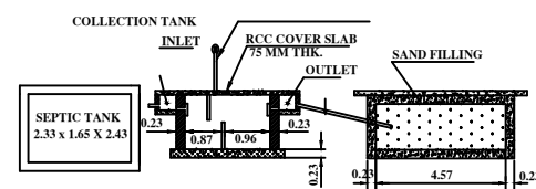
PLAN & SECTION ON SEPTIC TANK & DISP-TRENCH
