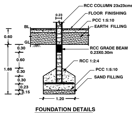
FOUNDATION DETAILS
