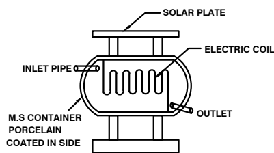
SOLAR SYSTEM
