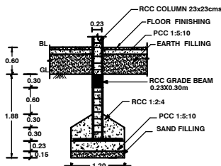
FOUNDATION DETAILS
