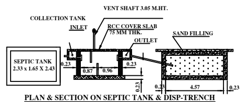
PLAN & SECTION ON SEPTIC TANK & DISP-TRENCH
