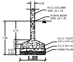
COLUMN FOUNDATION DETAILS
