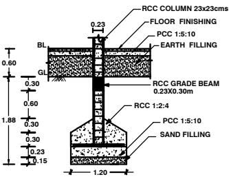
FOUNDATION DETAILS
