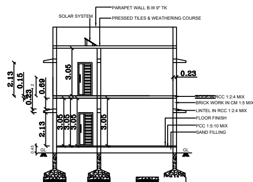
CROSS SECTION AB
