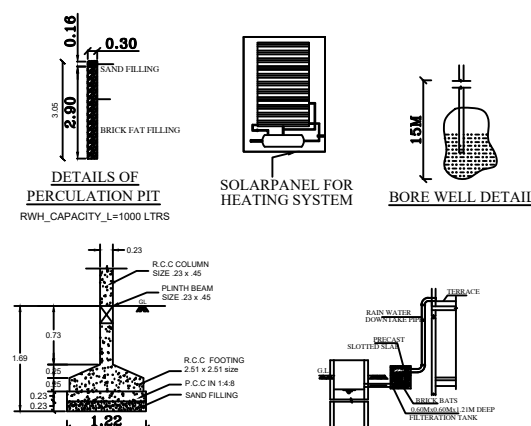
COLUMN FOUNDATION DETAILS
