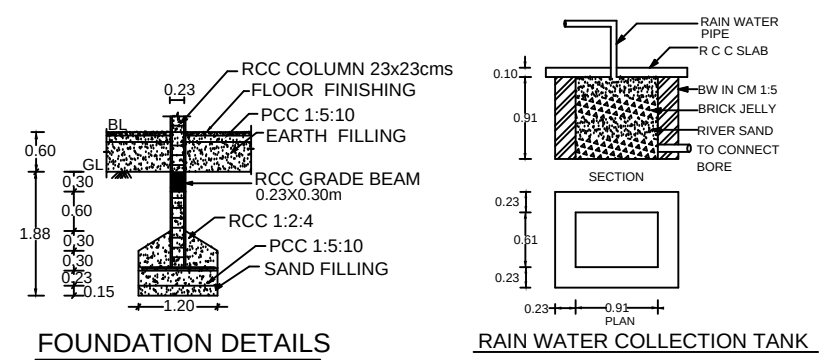
FOUNDATION DETAILS
