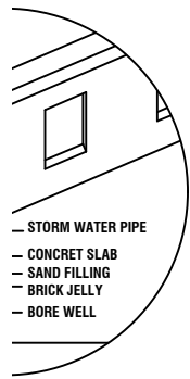
STORM WATER PIPE
