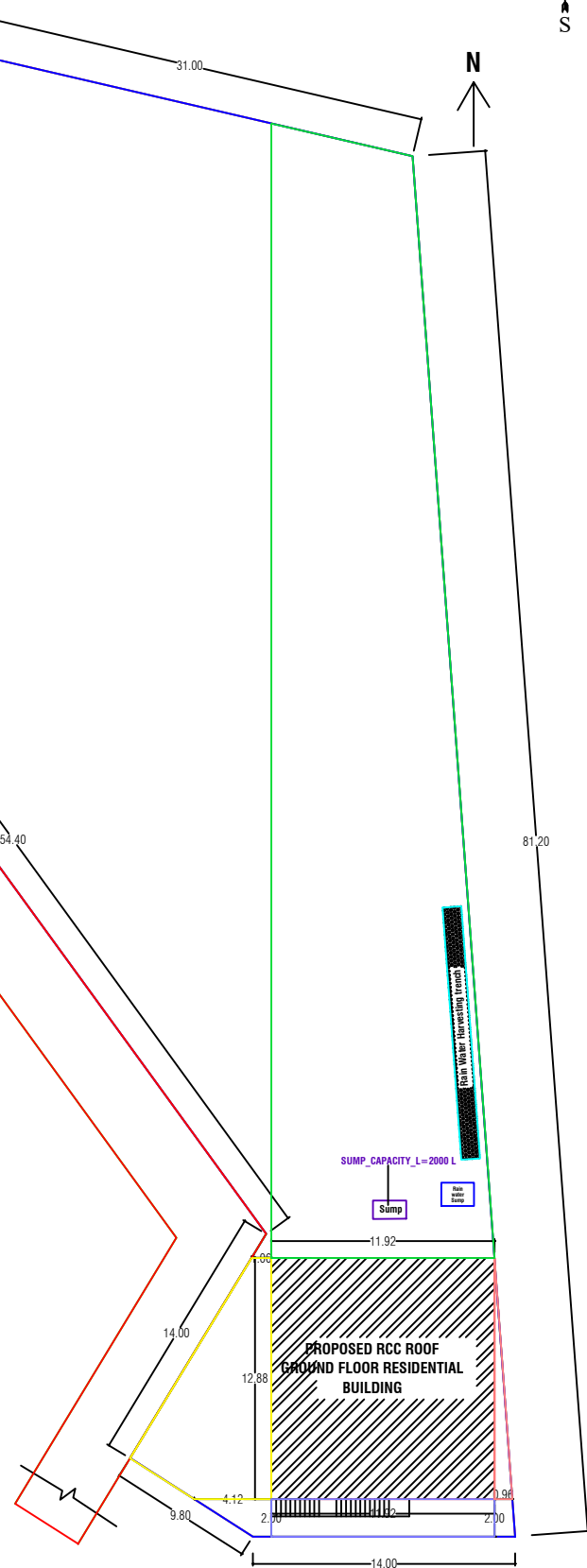
SITE PLAN [1 : 100]
