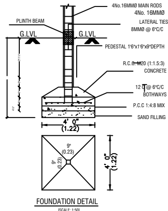
FOUNDATION DETAIL (SCALE: 1:50)
