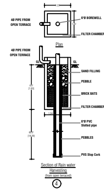
Section of Rain water Harvesting
