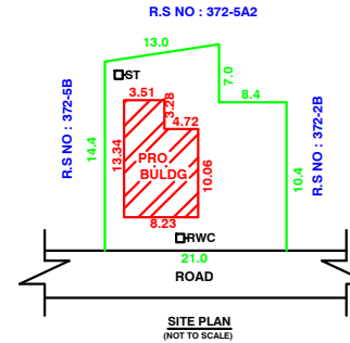
SITE PLAN (NOT TO SCALE)
