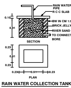
RAIN WATER COLLECTION TANK
