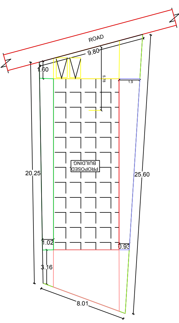
SITE PLAN
