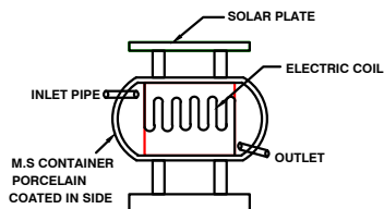
SOLAR SYSTEM
