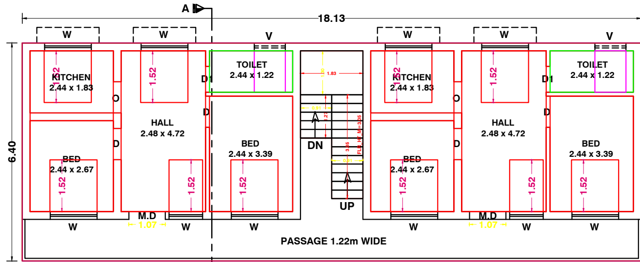
PRO. FIRST FLOOR PLAN
