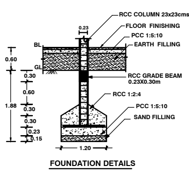
FOUNDATION DETAILS
