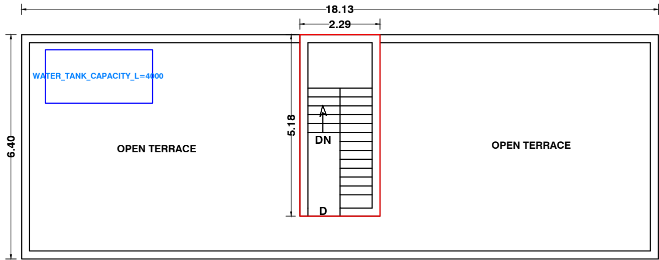
PRO. HEAD ROOM PLAN
