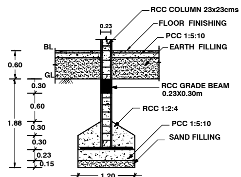
FOUNDATION DETAILS
