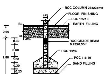
FOUNDATION DETAILS
