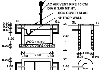
PLAN AND CROSS SECTION OF ST&SP.
