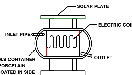
SOLAR SYSTEM
