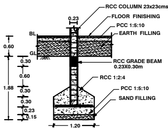
FOUNDATION DETAILS
