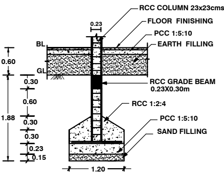
FOUNDATION DETAILS
