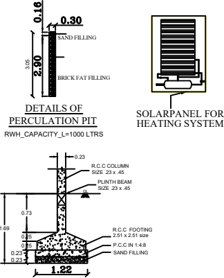
COLUMN FOUNDATION DETAILS
