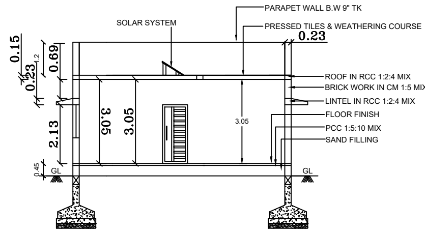
CROSS SECTION AB
