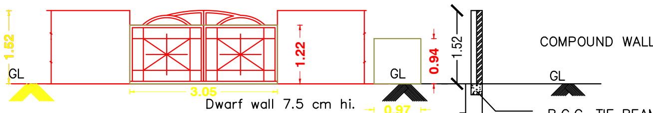
COMPOUND WALL DETAILS
