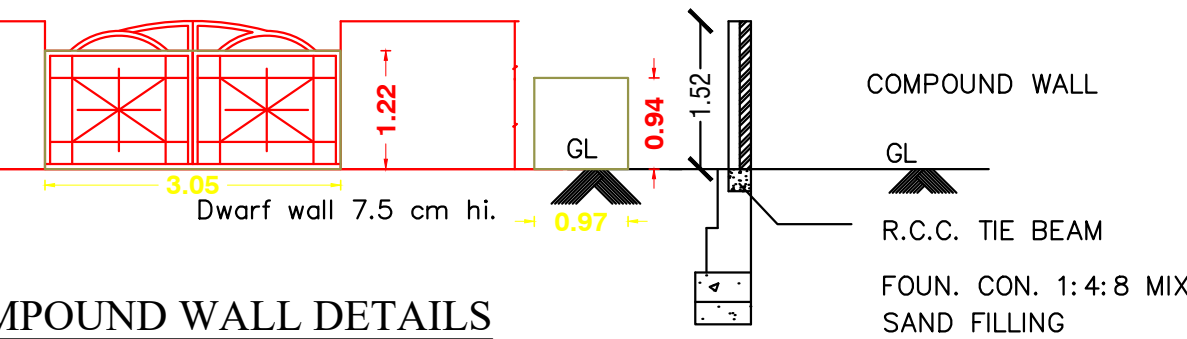
SECTION
