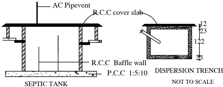
SECTION
